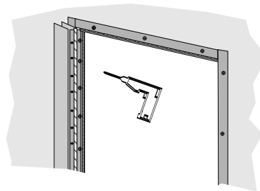
FIG.3 INSTALLATION OF HEADER, SIDE Z-BARS & HINGE CHANNEL
